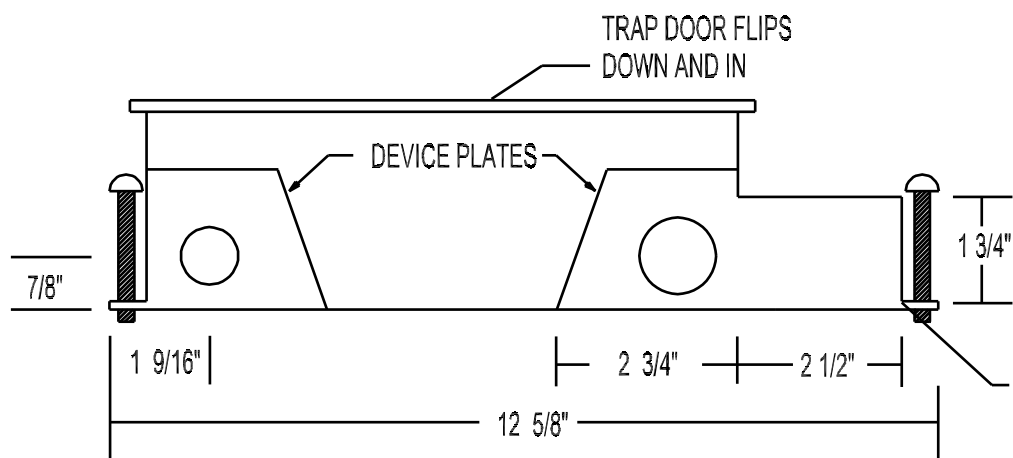
END VIEW
