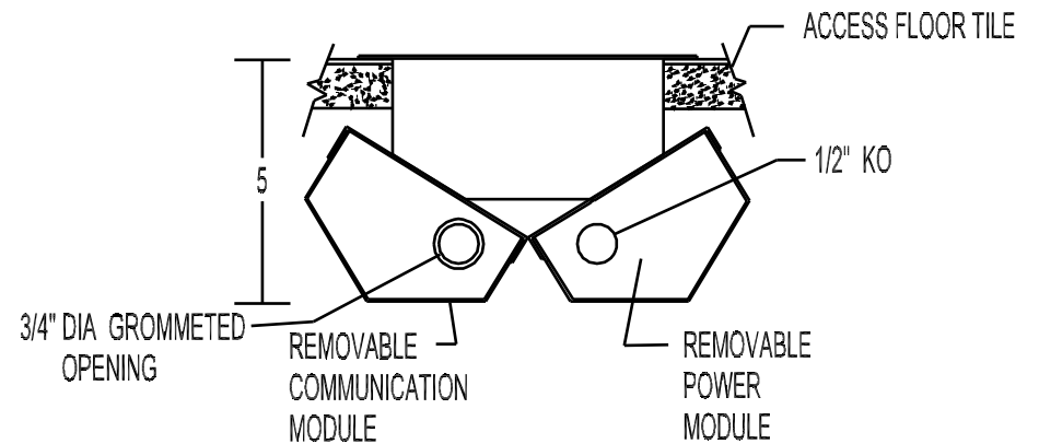
END SECTION
