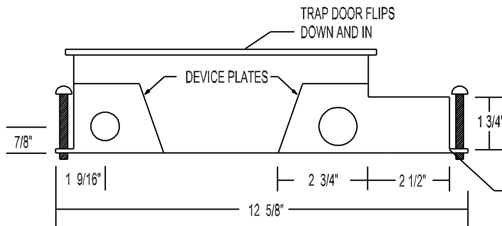
END VIEW
