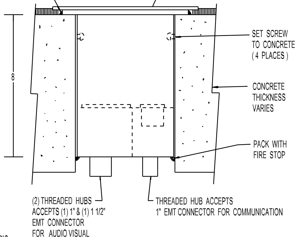
SIDE SECTION
