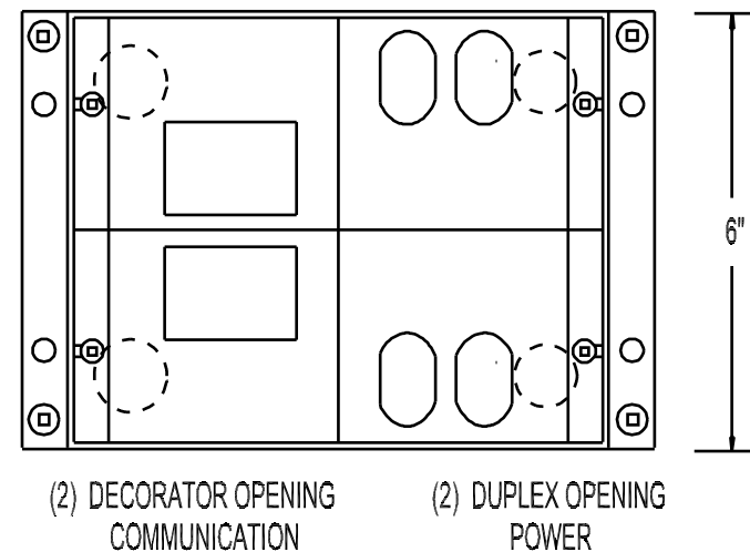
TOP VIEW INSIDE BOX
