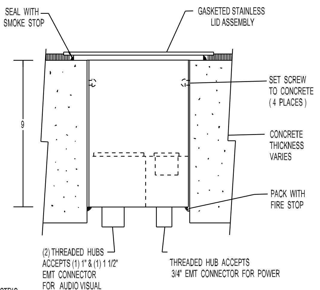
SIDE SECTION
