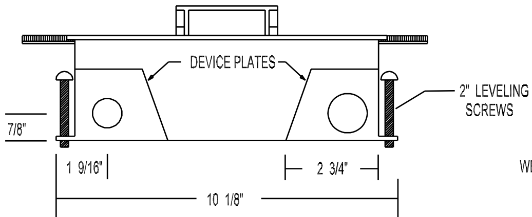
END VIEW
