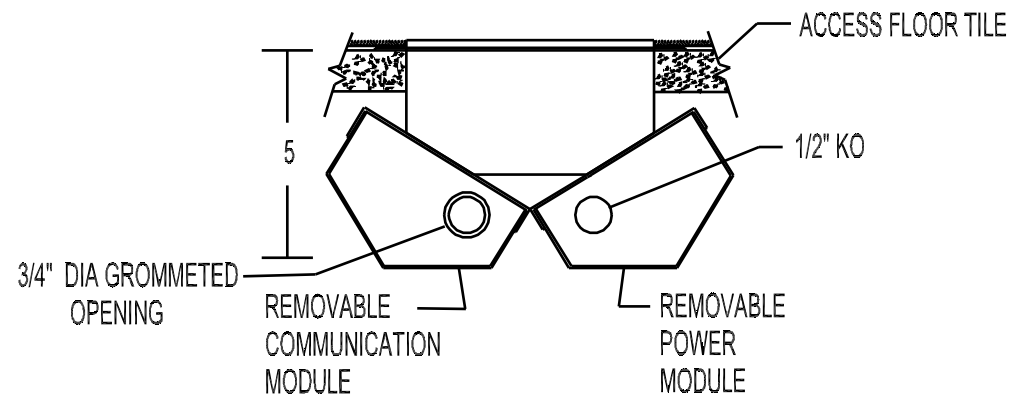
END SECTION
