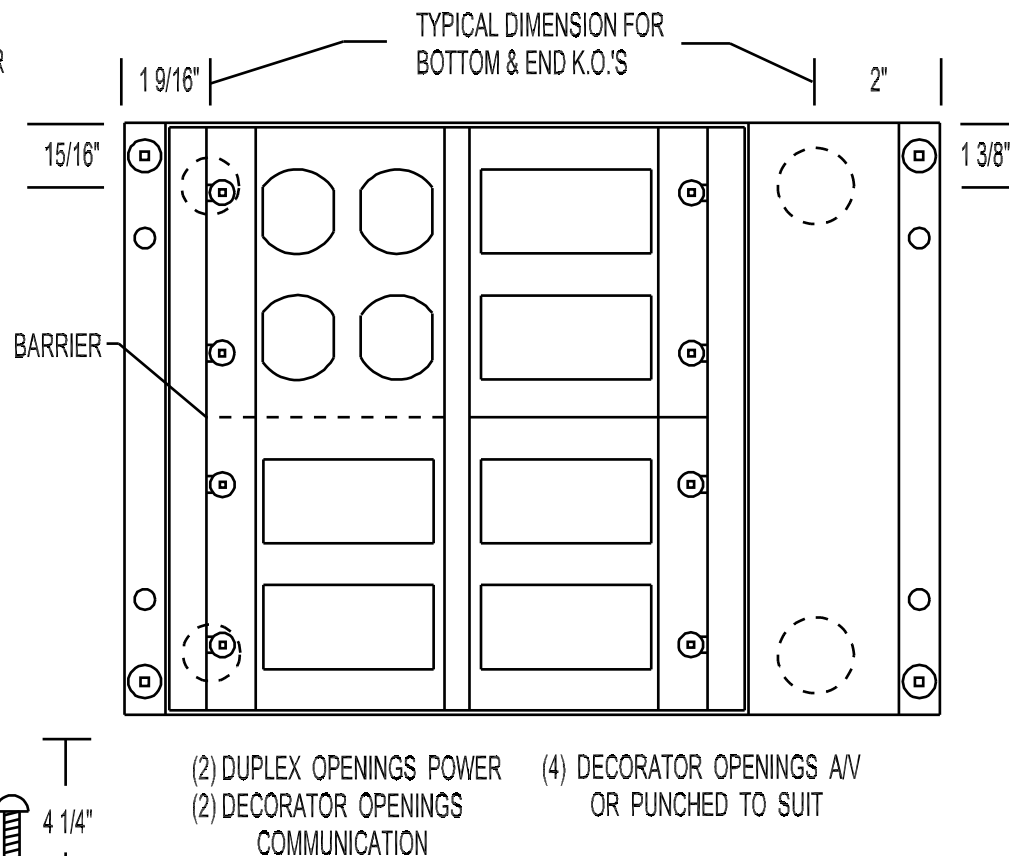
TOP VIEW INSIDE BOX
