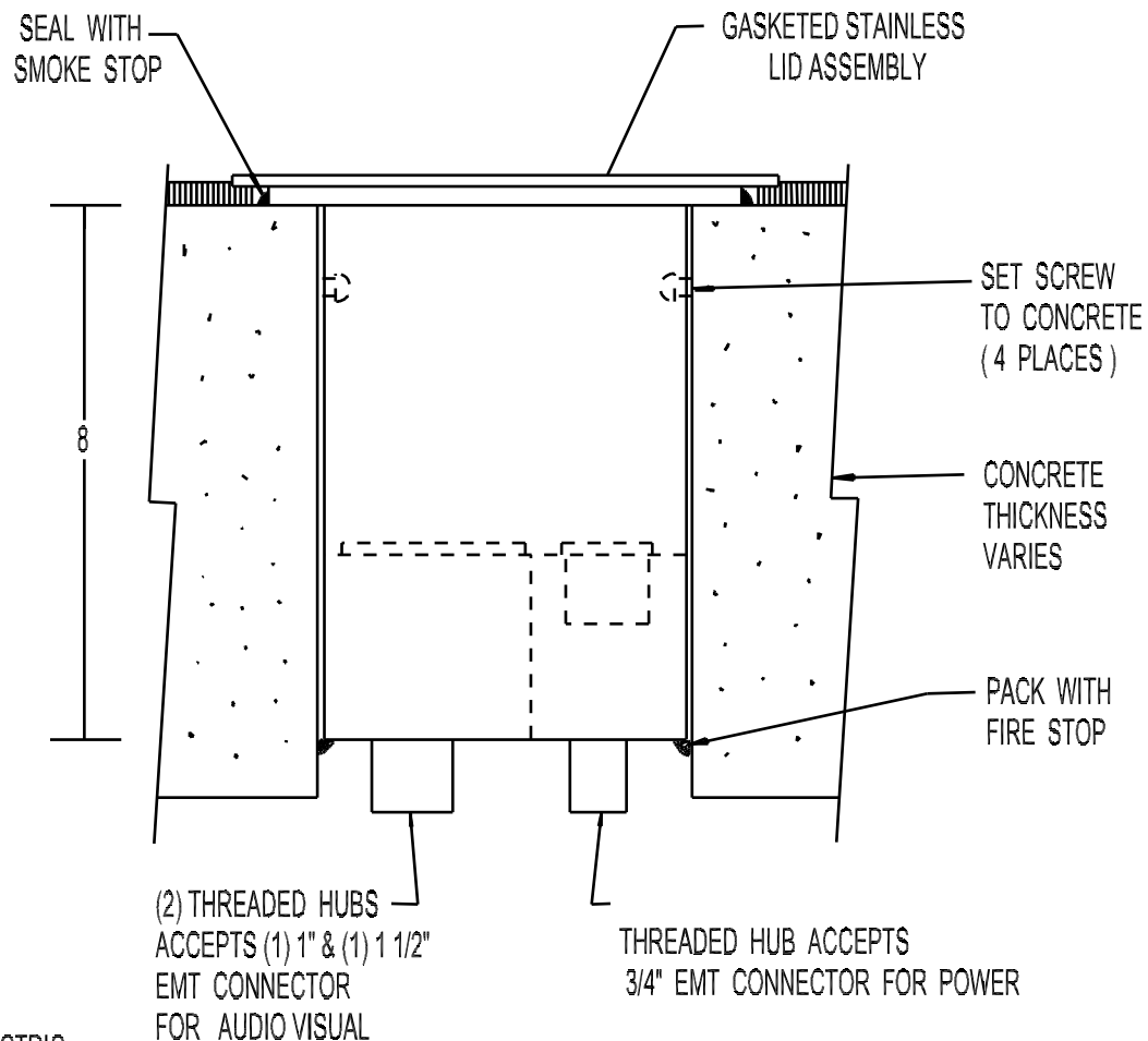
SIDE SECTION
