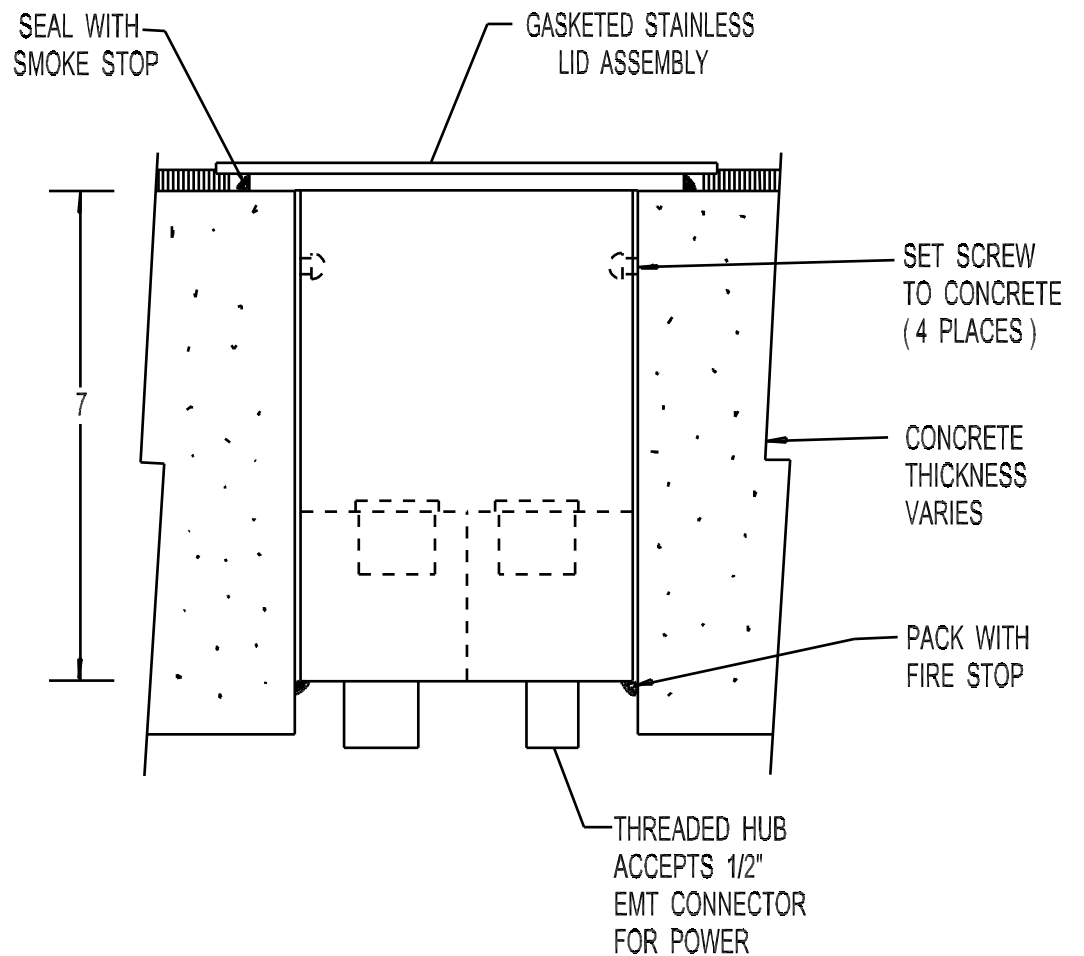
SIDE SECTION
