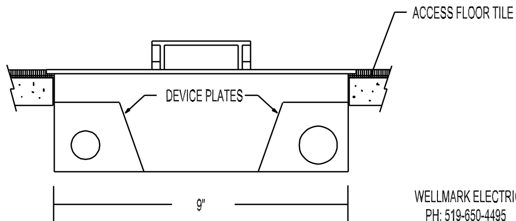
END VIEW
