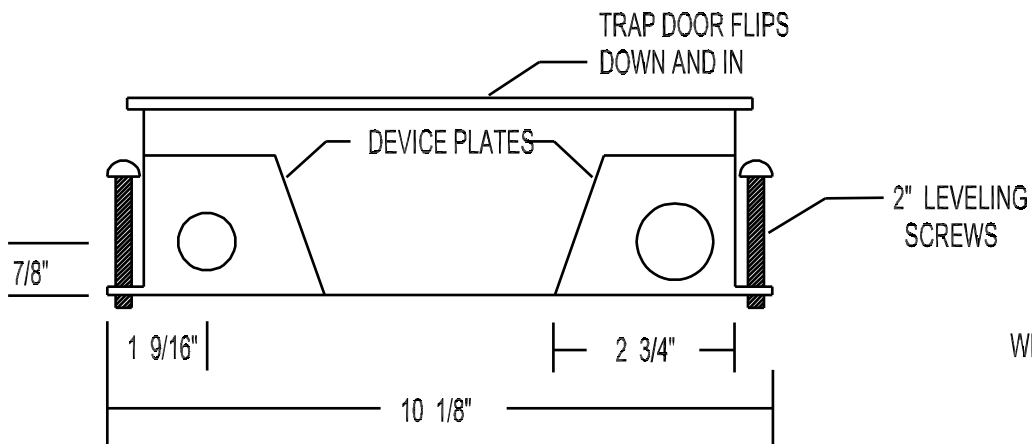
END VIEW
