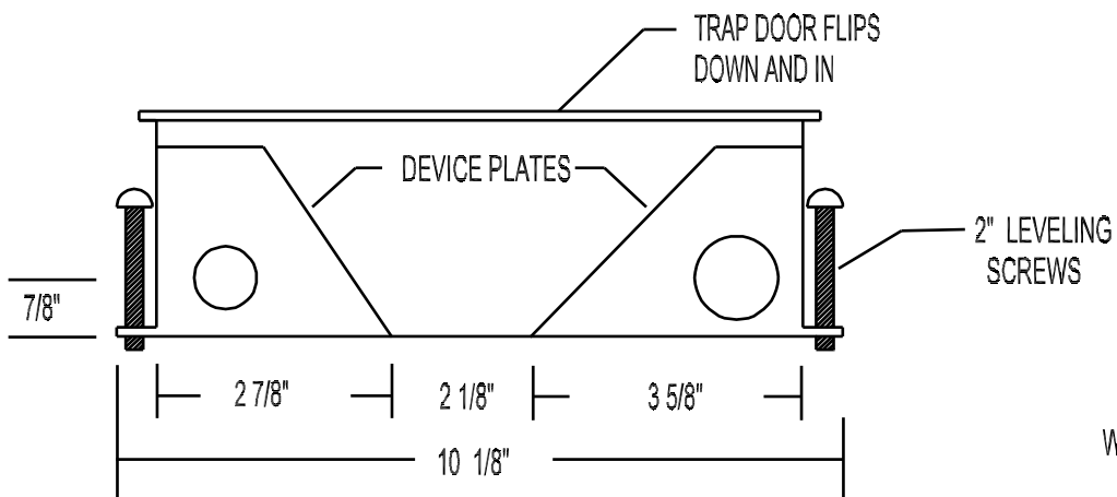
END VIEW
