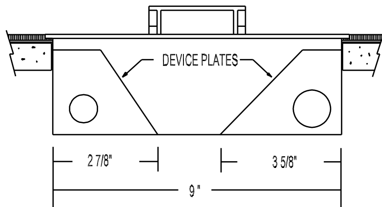
END VIEW
