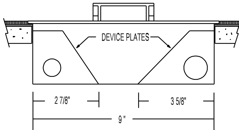
END VIEW
