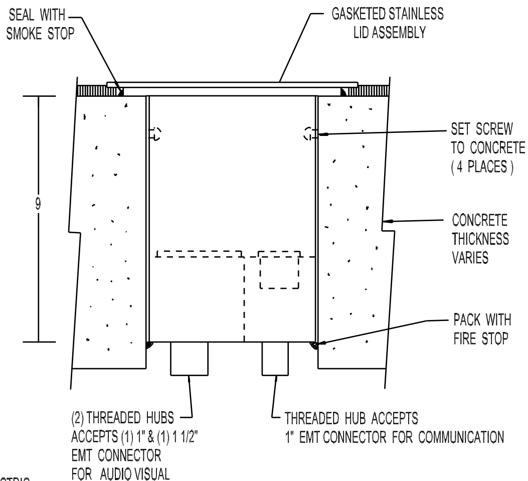
SIDE SECTION
