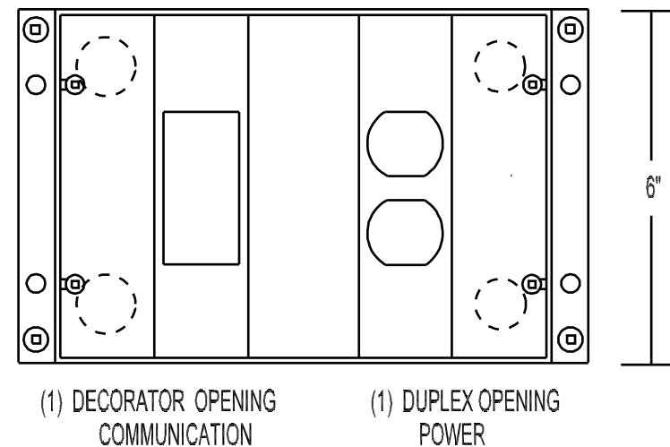
TOP VIEW INSIDE BOX
