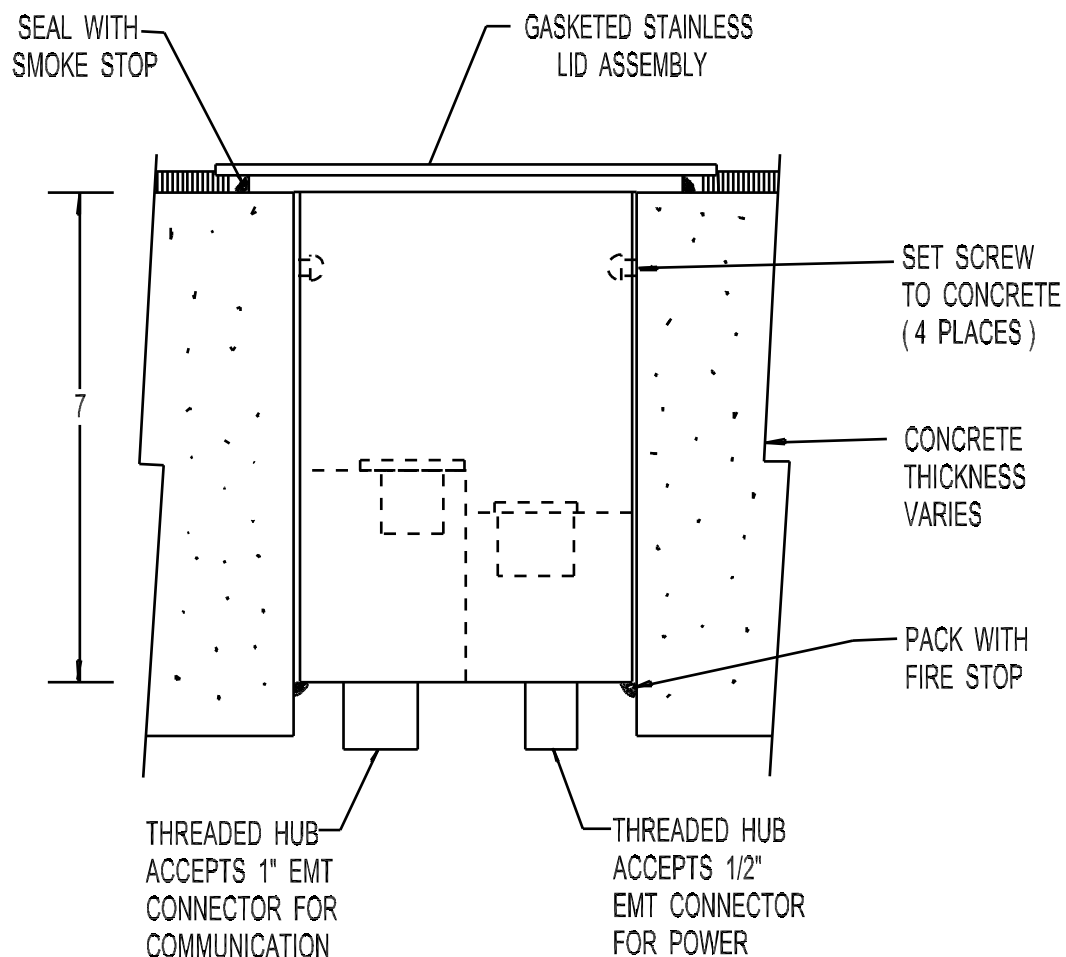
SIDE SECTION
