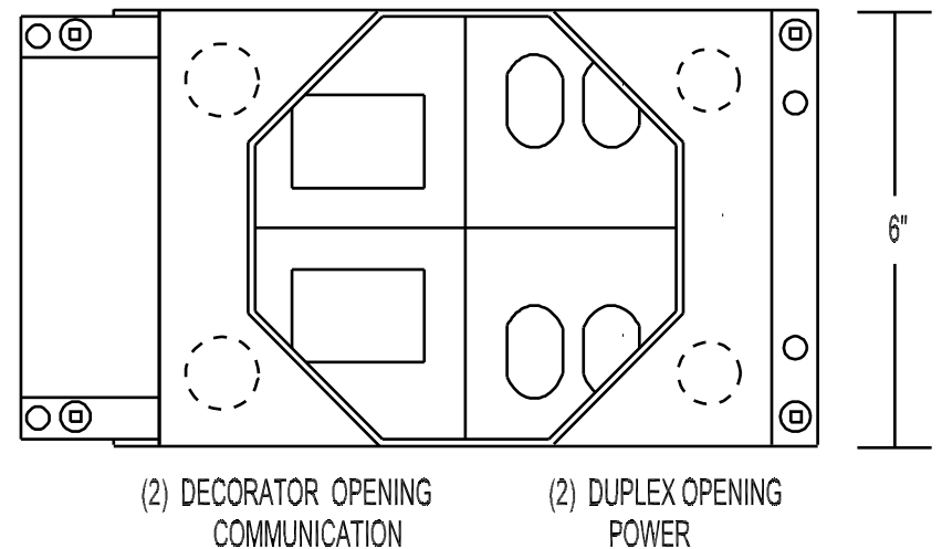
TOP VIEW INSIDE BOX
