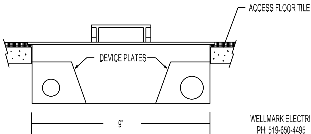
END VIEW
