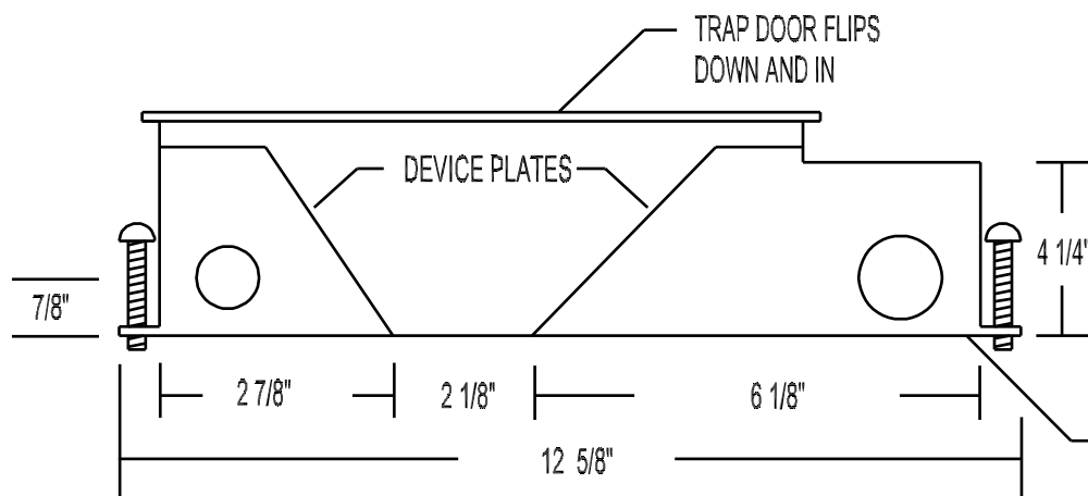
END VIEW
