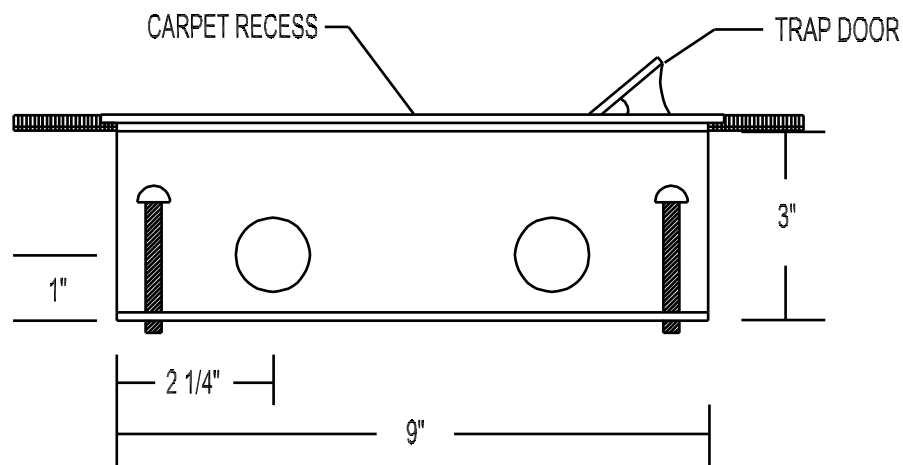
SIDE VIEW
