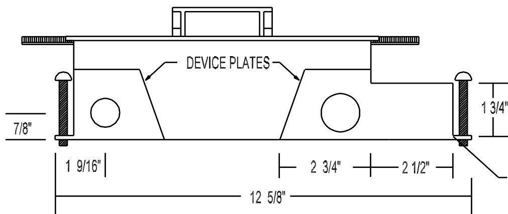
END VIEW
