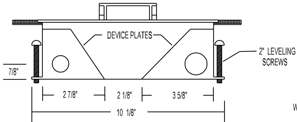
END VIEW
