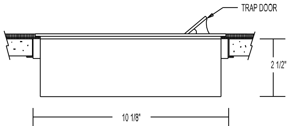
SIDE VIEW
