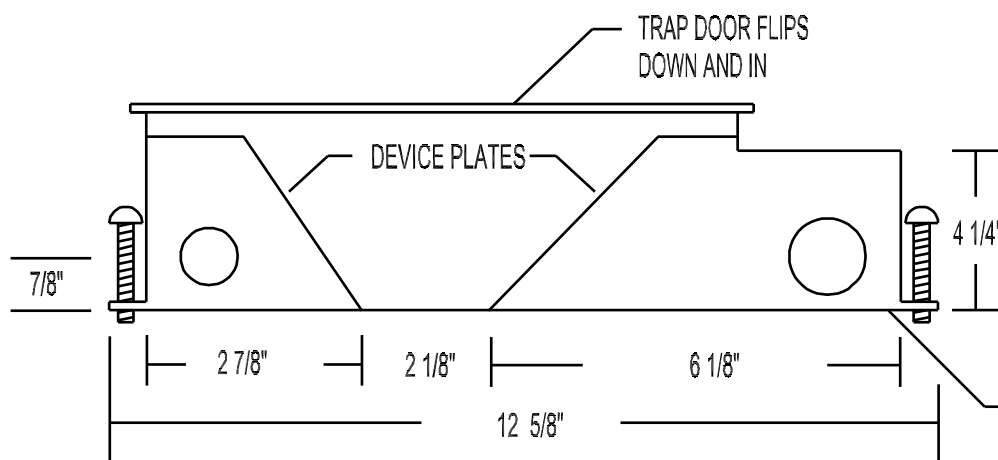
END VIEW
